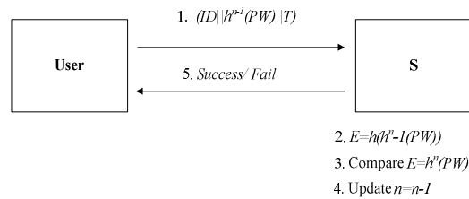
Figure 4. Login to Server
