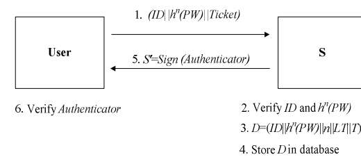
Figure 3. Registration to Server
