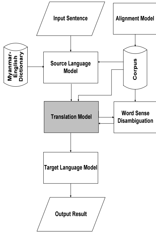
Figure 1. Machine translation system of Myanmar to English
