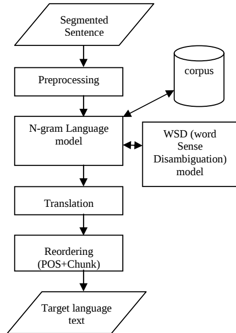
Figure 2. System Architecture of Translation Model
