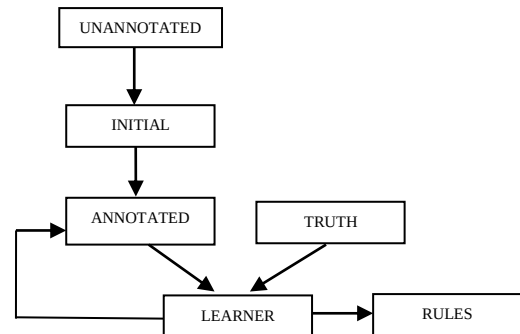
Figure 1. Transformation-based learning
