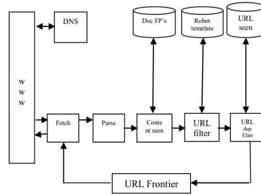
Figure 1. Architecture of a Basic Web Crawler [3]
