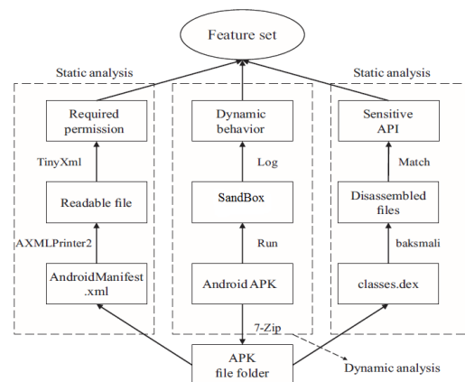
Figure 2. Proposed Feature Extraction for apk
