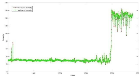
Figure 3. Estimated and measured intensity values of one pixel through video sequences
