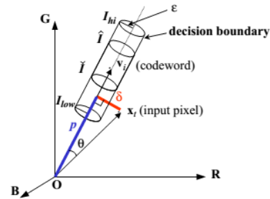
Figure 1. Cylinder color model of Codebook algorithm
